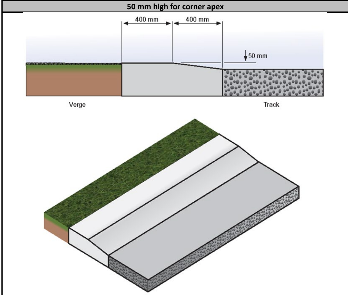
Figure 4 Type 3 Bevelled Kerb
