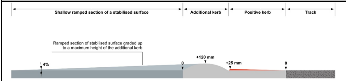
Figure 5 Type 4 Combination Kerb
