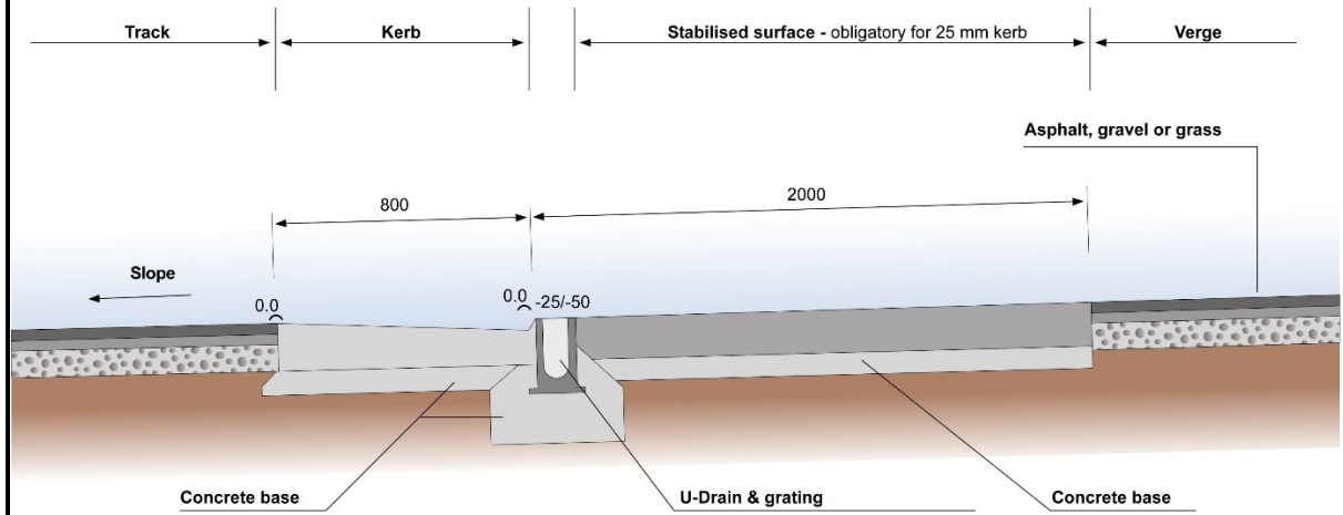
Figure 3 Type 2 Melbourne Kerb (Detail)
